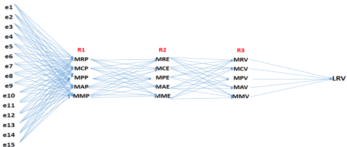
Figure 1. Neural networks (Multilayer Perceptron) of the learned meaning of violence
